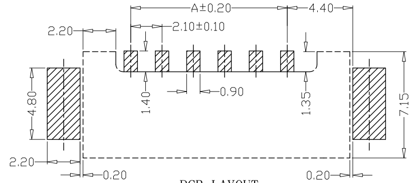
PCB LAYOUT
